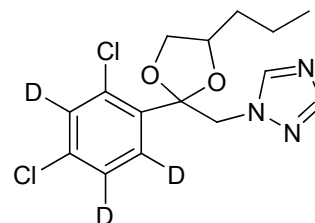
Propiconazole-D3
